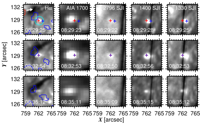
Figure 2. Time evolution of EB-1 in various diagnostics. Left to right: co-spatial image cutouts of CRISP H \alpha wings, AIA 1700 Å, IRIS Mg II k, Si IV, and C II slitjaws. The red and blue contours in the first column indicate patches of positive and negative polarity (thresholded at 0 and -1000 counts), respectively, based on the HMI line of sight magnetic field data. The time of observation is specified at the bottom of each panel. The plus signs mark the locations for which corresponding spectra are shown with the same color coding in Figure 4. The cyan circle indicates the size (and instantaneous location) of the mask used to determine the light curves in Figure 3. The arrow in the same panel specifies the “upright” direction to the nearest limb. The panels in each column have been byte-scaled to the same extremes.
