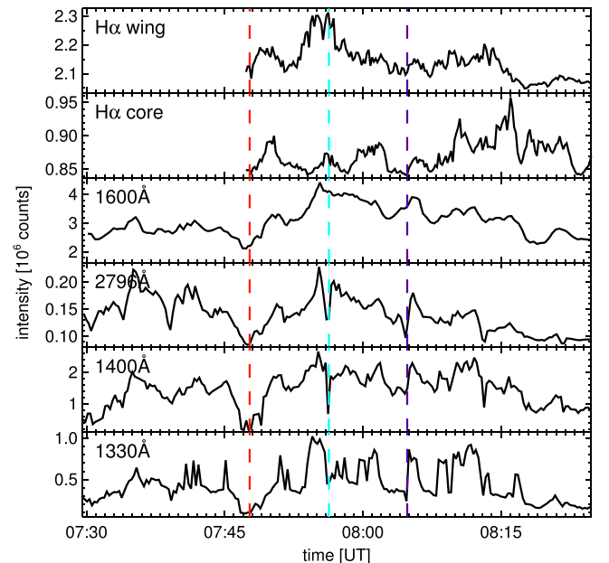
Figure 7. Light curves for EB-2 in the format of Figure 3. In this case, the integration aperture had a diameter of 3.5 arcsec (1.5 times the maximum diameter of the H\alpha EB detection contour), as indicated in the first panel of Figure 6. The three dashed vertical lines correspond to the sampling times of the three rows in Figure 6. There are corresponding dips in the lower three curves from the slit presence over the feature.
